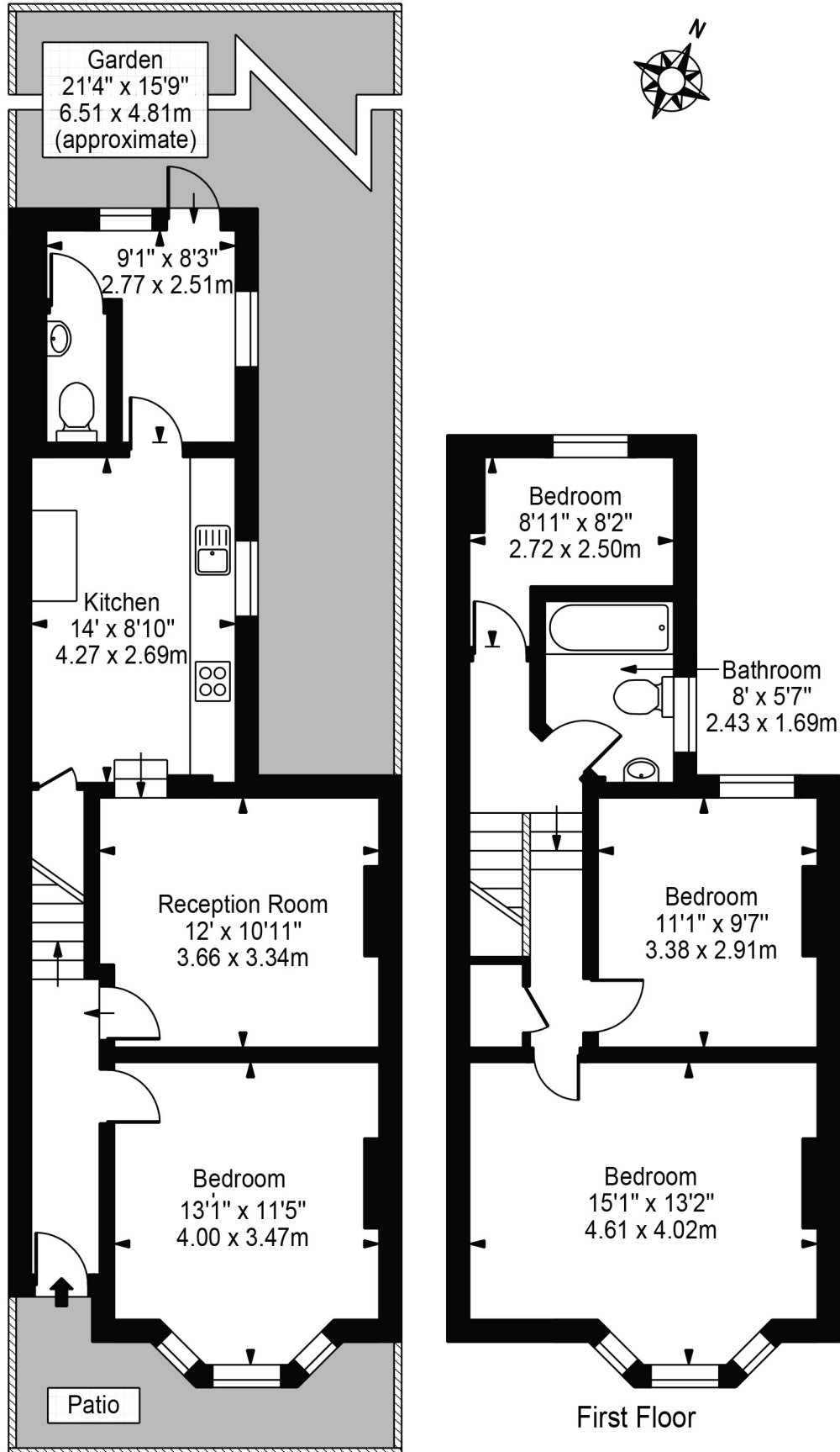
Ground Floor
