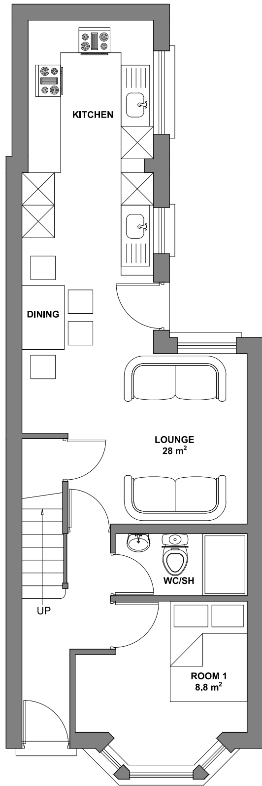
① PLAN - GROUND FLOOR
